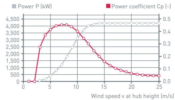
Calculated power curve
