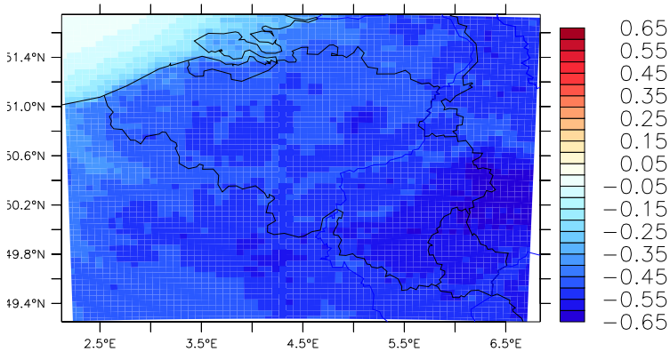
MAR-MIRr8.5 (2006-2100)
