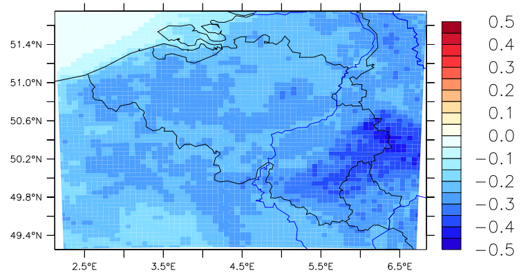
MAR-NORr8.5 (2006-2100)
