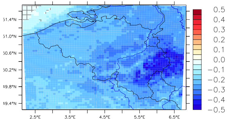
MAR-MIRrcp8.5 (2006-2100)
