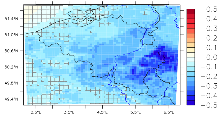
MAR-NORrcp8.5 (2006-2100)
