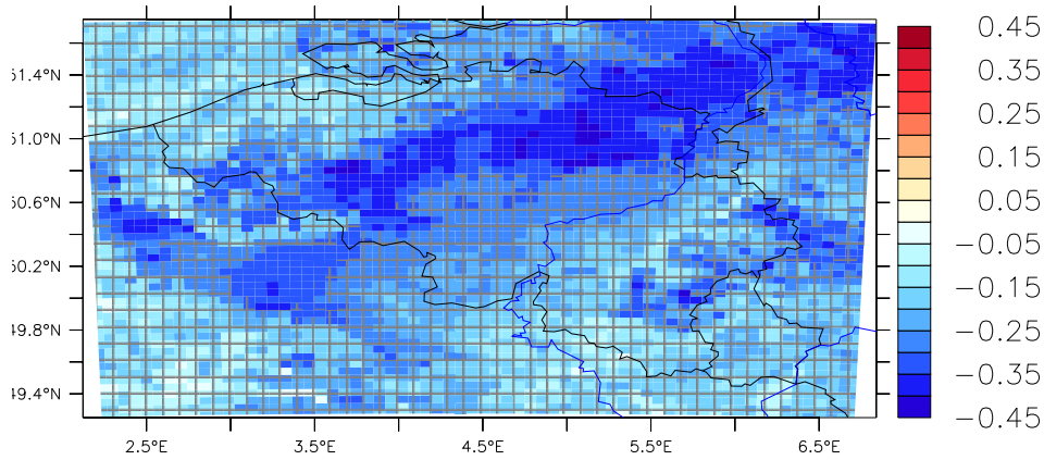
MAR-ERAint (1958-2016)
