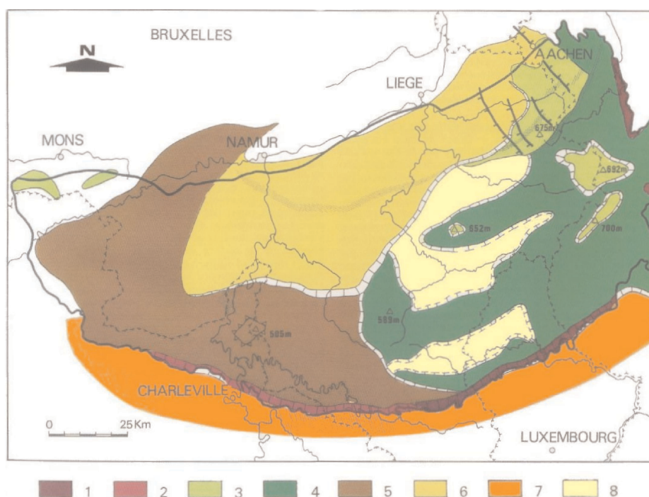
Fig. 1.- Paleosurfaces in the Ardenne-Eifel before the Plio-Pleistocene downcutting (taken from Demoulin, 1995). 1. pre-Triassic surface. 2. post-Hercynian surface. 3. pre-Senonian surface. 4. Dano-Montian surface. 5. Eocene surface. 6. Pre-Tongrian surface. 7. Eocene/Oligocene surface of the NE Paris basin. 8. Oligo-Miocene planation basins. - Hatched zones between the surfaces: erosion scarps. - Stippled band: flexure zone.
